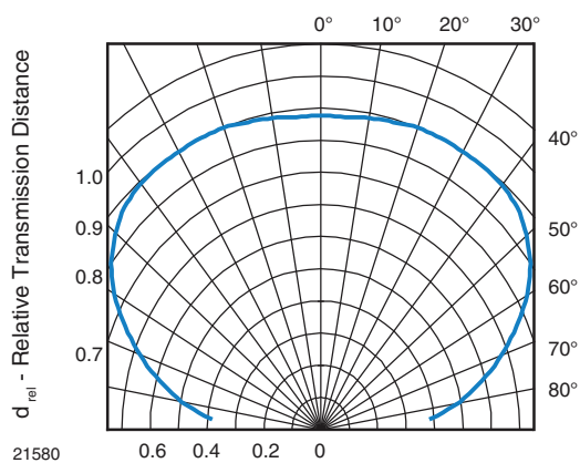
Fig. 12 - Vertical Directivity
