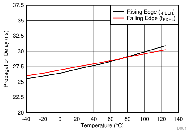
Figure 7-18. Propagation Delay, Rising and Falling Edge
