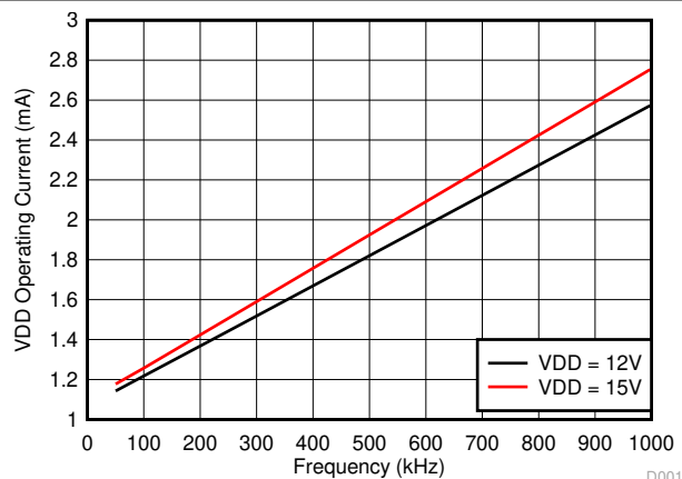
Figure 7-9. Per Channel Operating Current ( I_{VDDA/B} ) vs. Frequency
