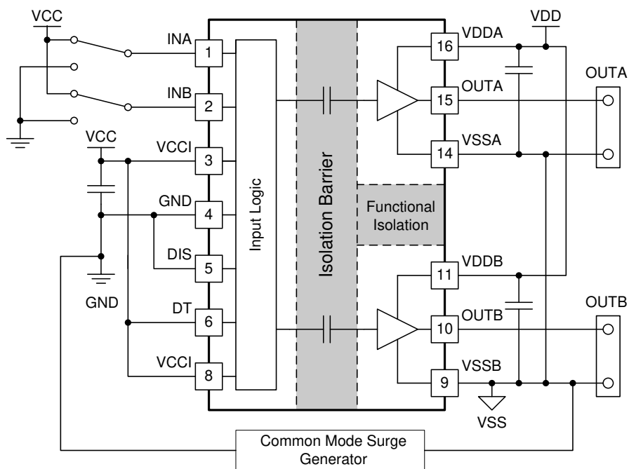
Figure 8-9. Simplified CMTI Testing Setup
