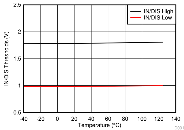
Figure 7-16. INA/INB/DIS High and Low Threshold Voltage
