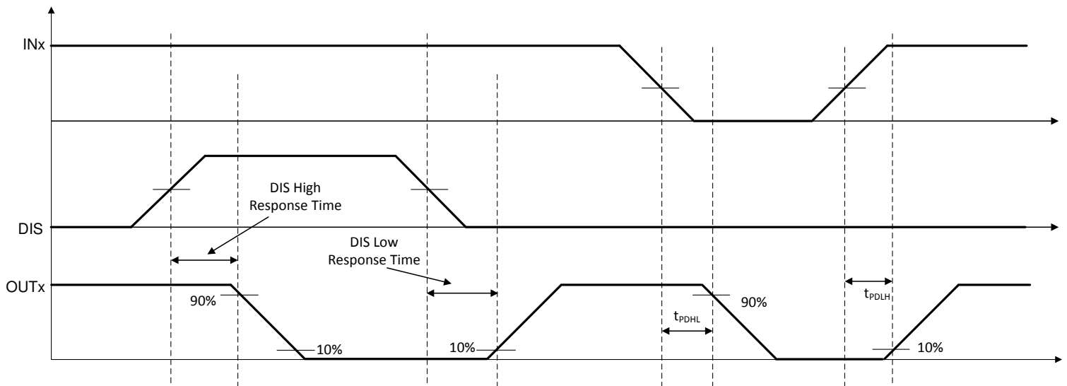
Figure 8-5. Disable Pin Timing
