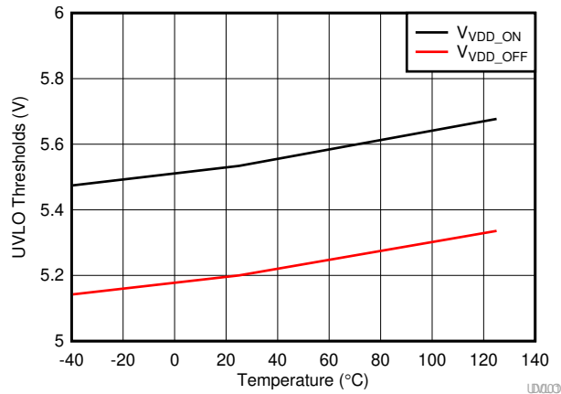
Figure 7-26. 5-V VDD UVLO Threshold Voltage
