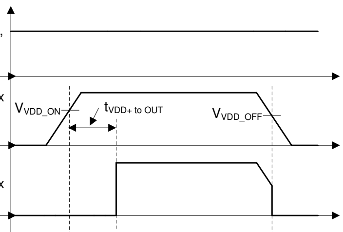
Figure 8-8. VDDA/B Power-up UVLO Delay
