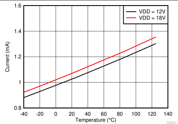
Figure 7-5. VCCI Operating Current - I_{VCCI}
