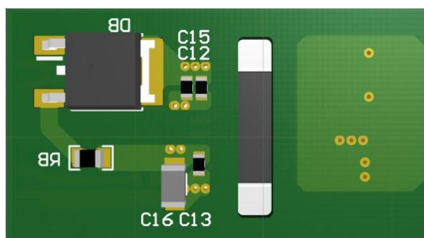
Figure 12-5. 3-D PCB Bottom View
