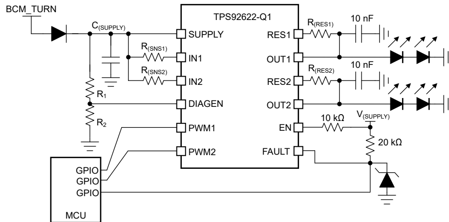
Figure 7-4. Typical Application Schematic
