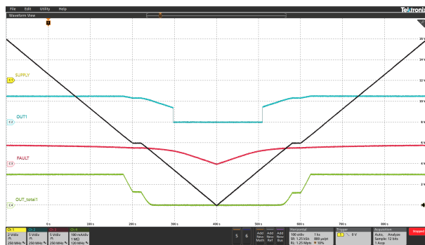
Figure 5-19. Transient Overvoltage
