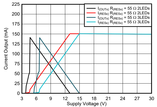
Figure 5-8. Output Current Distribution vs Supply Voltage
