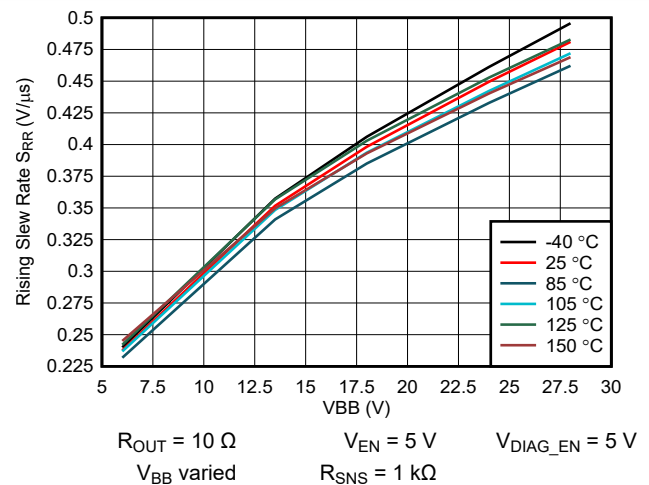
Figure 6-16. Rising Slew Rate SRR vs Temperature
