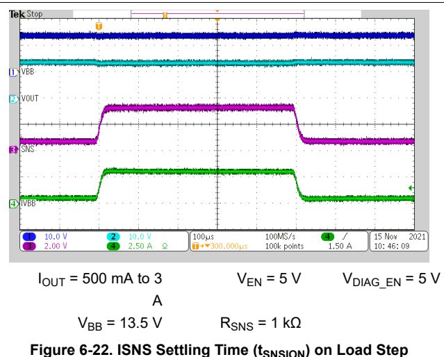
Figure 6-22. ISNS Settling Time ( t_{SNSION} ) on Load Step
