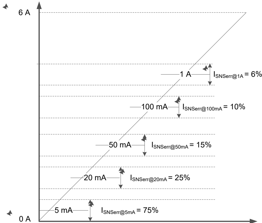
Figure 8-1. Current-Sense Accuracy
