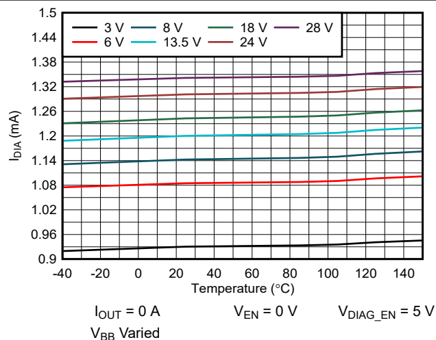
Figure 6-5. Diagnostic Current I_{DIA} vs Temperature
