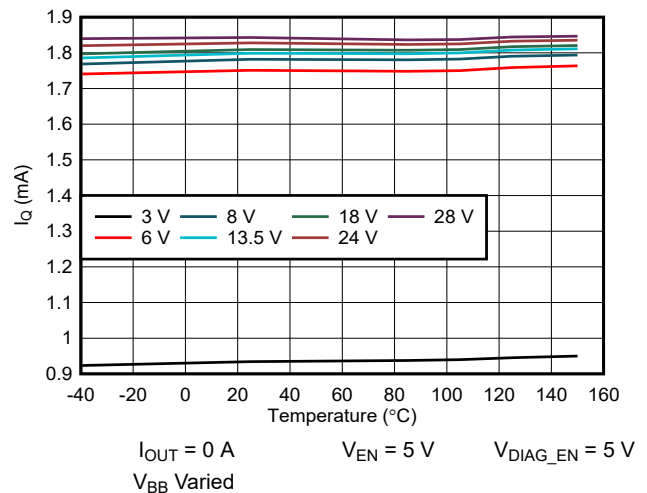
Figure 6-4. Quiescent Current I_Q vs Temperature
