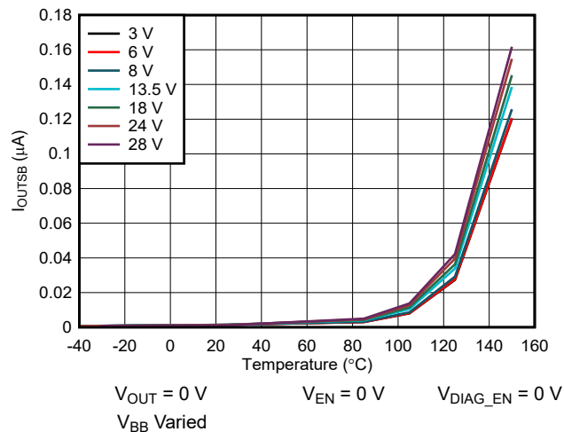
Figure 6-3. Output Leakage Current I_{OUT,STBY} vs Temperature
