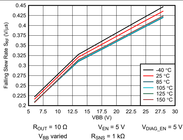
Figure 6-17. Falling Slew Rate SRF vs Temperature
