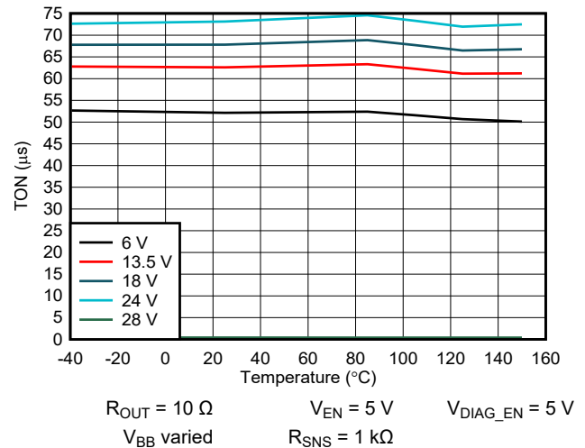
Figure 6-14. Turn on time T_{ON} vs Temperature
