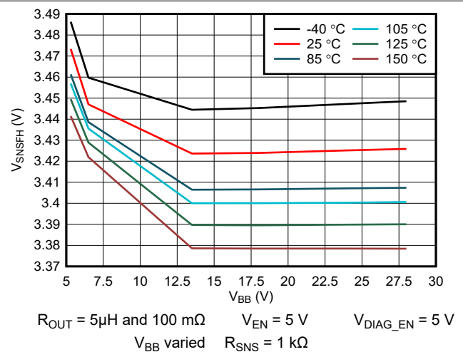
Figure 6-12. V_{SNS(FH)} (3.3\text{ V}) vs V_{BB}
