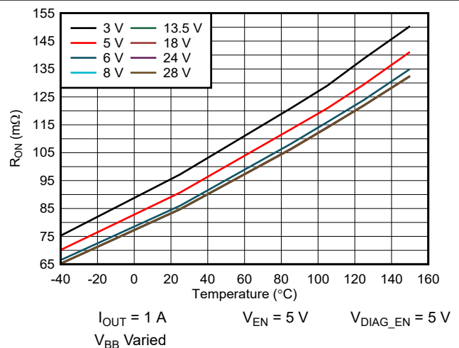
Figure 6-6. R_{DS(on)} vs Temperature
