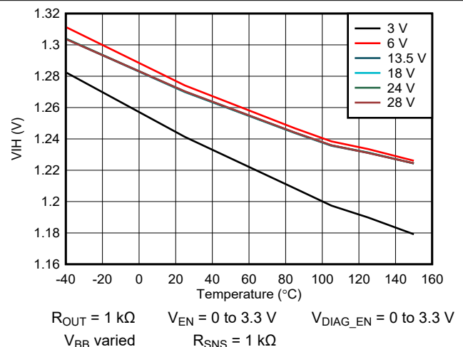
Figure 6-18. V_{IH} vs Temperature
