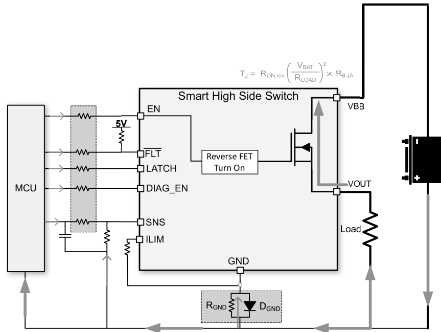
Figure 8-21. Reverse Protection With GND Network
