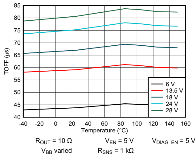
Figure 6-15. Turn off time T_{OFF} vs Temperature
