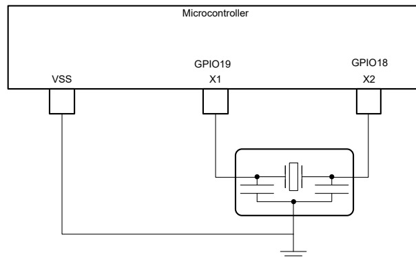
Figure 6-15. External Resonator
