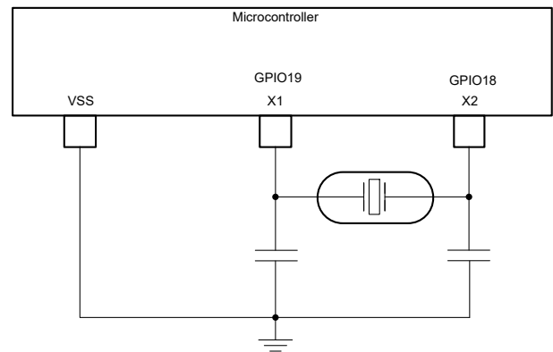
Figure 6-14. External Crystal
