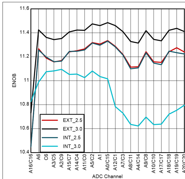
Figure 6-40. Per-Channel ENOB for 80-Pin PN LQFP and 64-Pin PM LQFP
