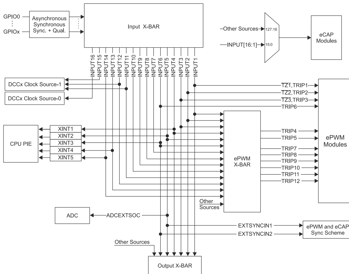
Figure 5-5. Input X-BAR
