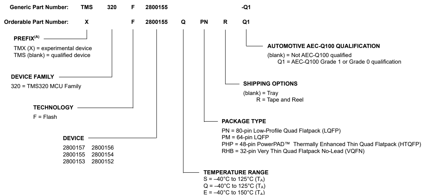
Figure 9-1. Device Nomenclature
