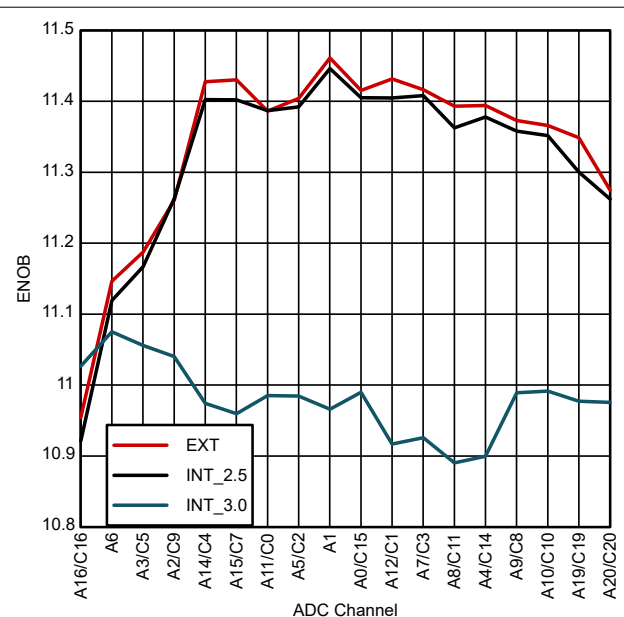
Figure 6-41. Per-Channel ENOB for 48-Pin PHP HTQFP
