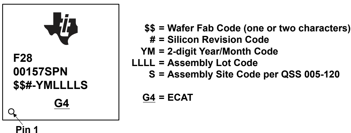
Figure 9-2. Package Symbolization for PN Package
