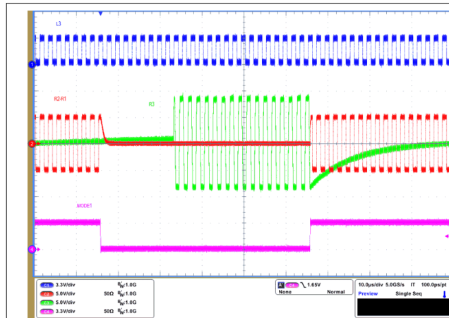
Figure 8-12. RS-232 to RS-485 Mode Switching Waveform
