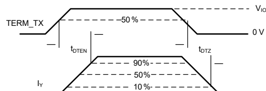
Figure 6-10. Termination Resistor Switching Measurement
