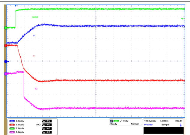
Figure 8-13. Mode Switching Waveform From Shutdown to RS-232 Mode
