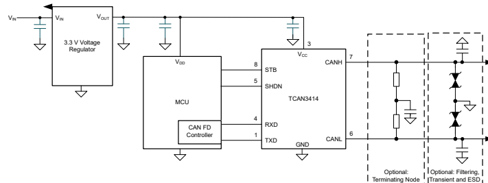
Simplified Schematic
