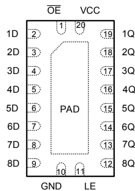
Figure 4-1. SN74ACT573-Q1 RKS Package, 20-Pin VQFN (Top View)
