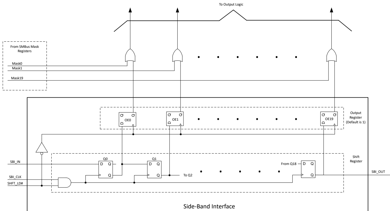
Figure 8-7. SBI Control Logic
