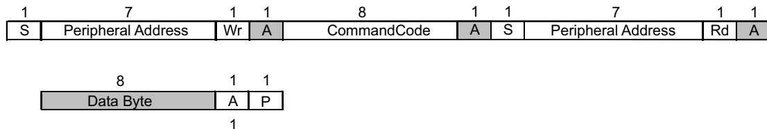
Figure 8-4. Byte Read Protocol
