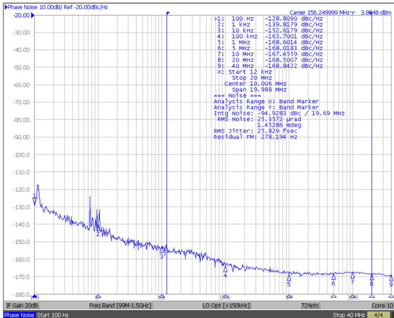
Figure 6-3. LMKDB Input Clock Phase Noise at 156.25 MHz
