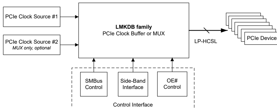
Figure 9-1. Typical Application
