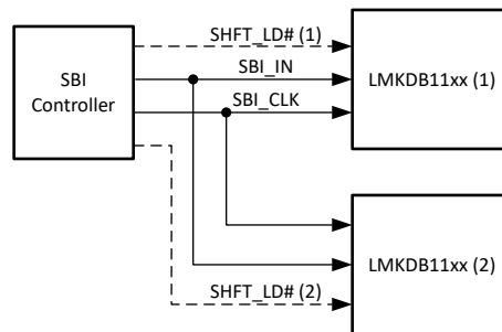
Figure 8-8. SBI Star Topology
