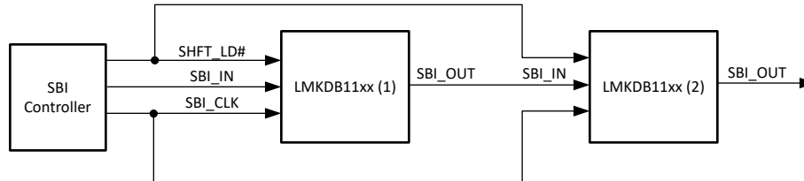
Figure 8-9. SBI Daisy Chain Topology
