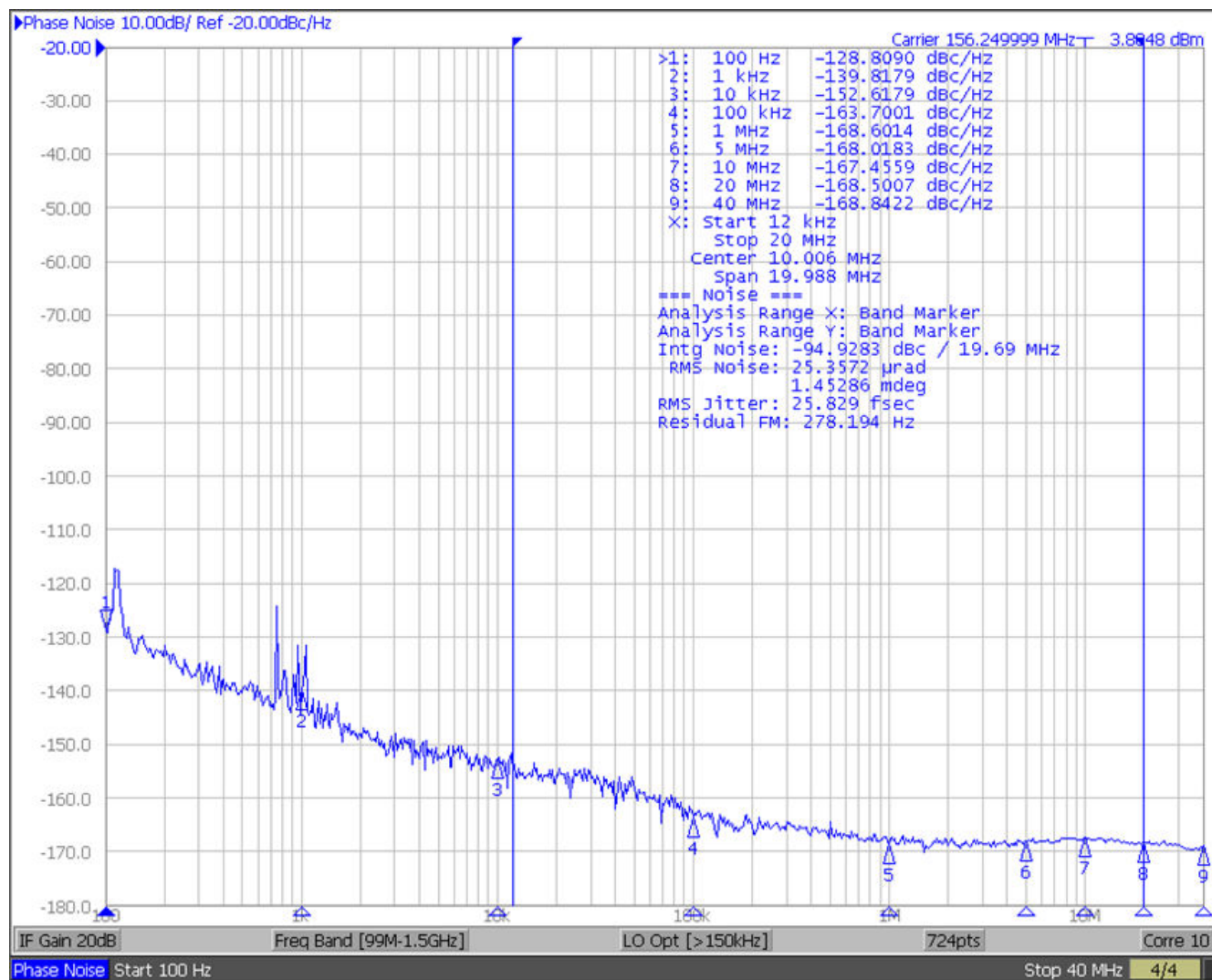
Figure 9-2. Reference Clock Phase Noise
