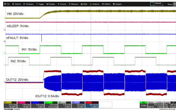
Figure 8-5. Device Power-up with Supply Voltage (VM)
