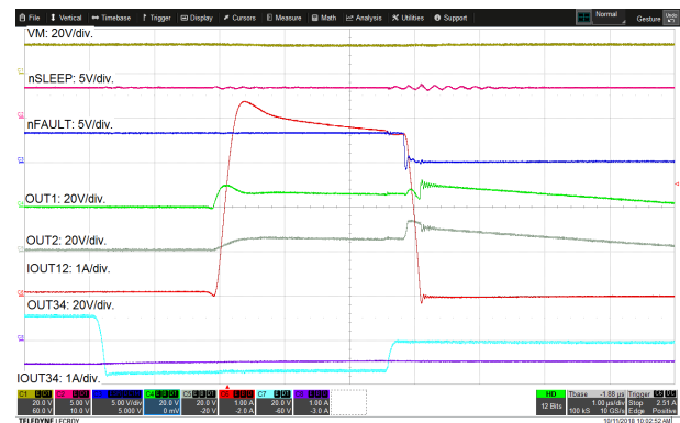
Figure 8-16. Zoomed Waveform of Over Current Protection
