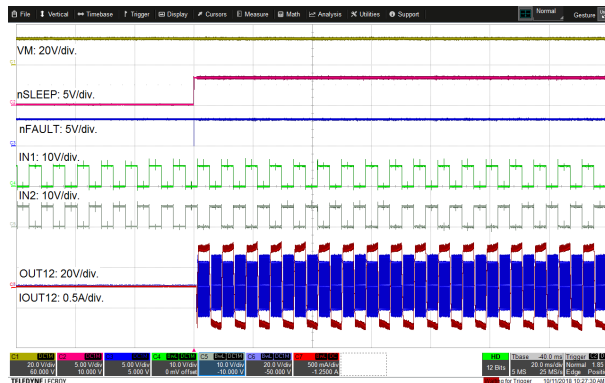
Figure 8-6. Device Power-up with nSLEEP
