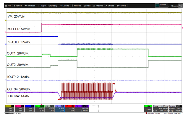
Figure 8-14. Open Load Detect Operation
