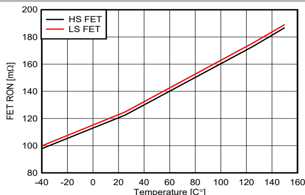
Figure 7-12. R_{HS\_ON} & R_{LS\_ON} vs Temperature at V_{VM} = 13.5 V
