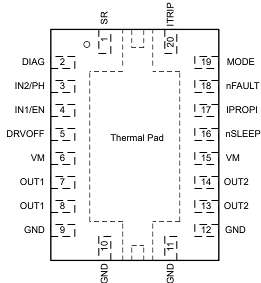
Figure 6-1. DRV8242H-Q1 HW variant in VQFN (20) package
