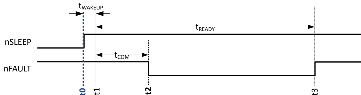
Figure 7-4. Wake-up from SLEEP State to STANDBY State Transition for HW Variant without ACK pulse
