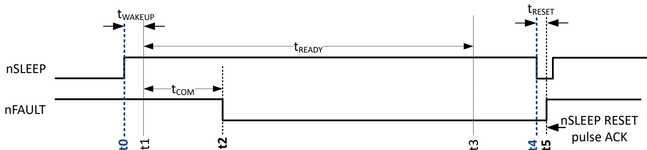
Figure 7-3. Wake-up from SLEEP State to STANDBY State Transition for HW Variant with ACK pulse
