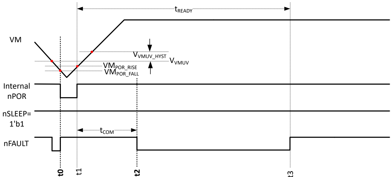
Figure 7-6. Power-up to STANDBY State Transition for HW Variant without ACK pulse
