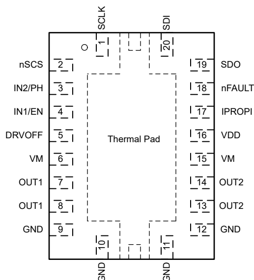
Figure 6-3. DRV8242P-Q1 SPI variant in VQFN (20) package
