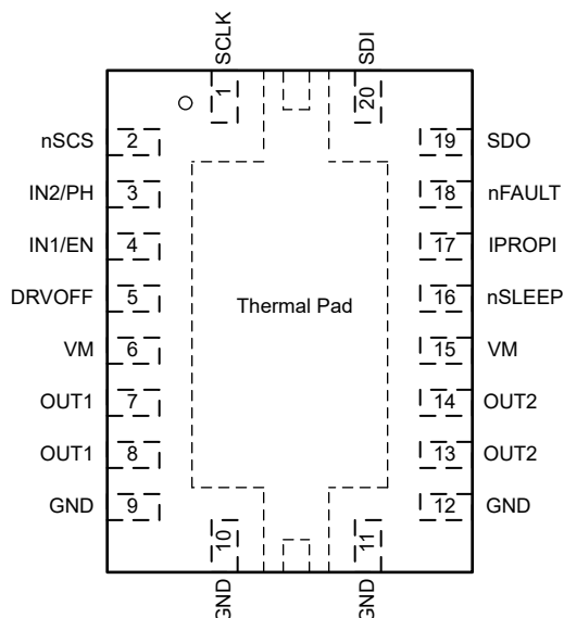
Figure 6-2. DRV8242S-Q1 SPI variant in VQFN (20) package
