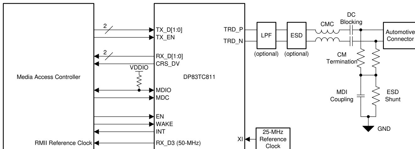
Figure 9-3. Typical Application (RMII Master)
