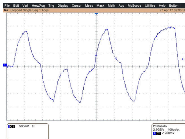
Figure 9-7. MDI IDLE Stream
