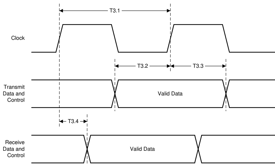
Figure 7-3. RMI Transmit and Receive Timing
