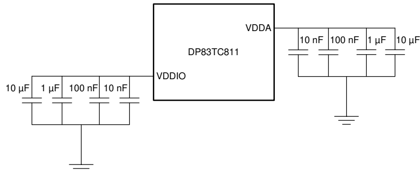
Figure 9-11. Recommended Supply De-Coupling Network
