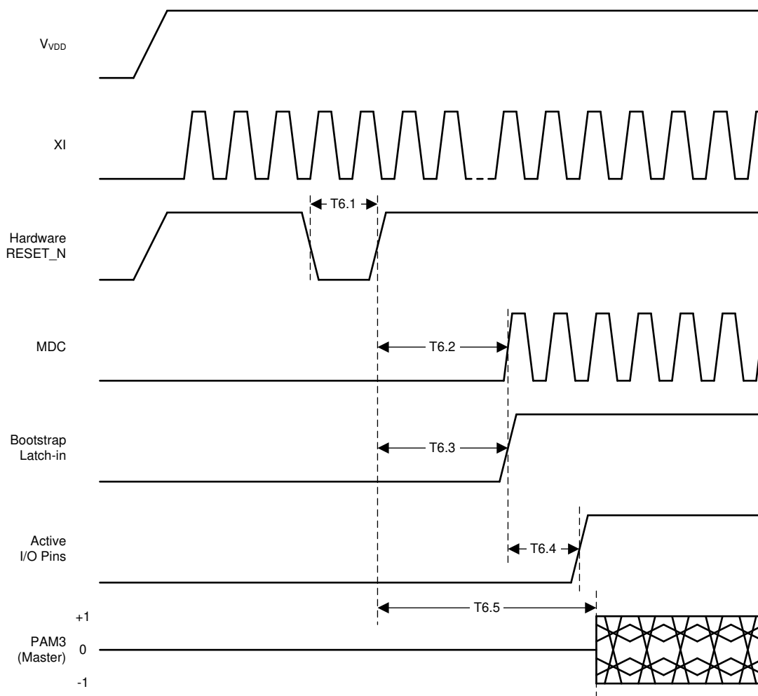
Figure 7-10. Reset Timing
