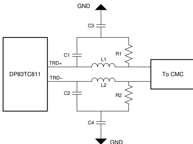
Figure 9-6. MDI Low-Pass Filter 1 2
