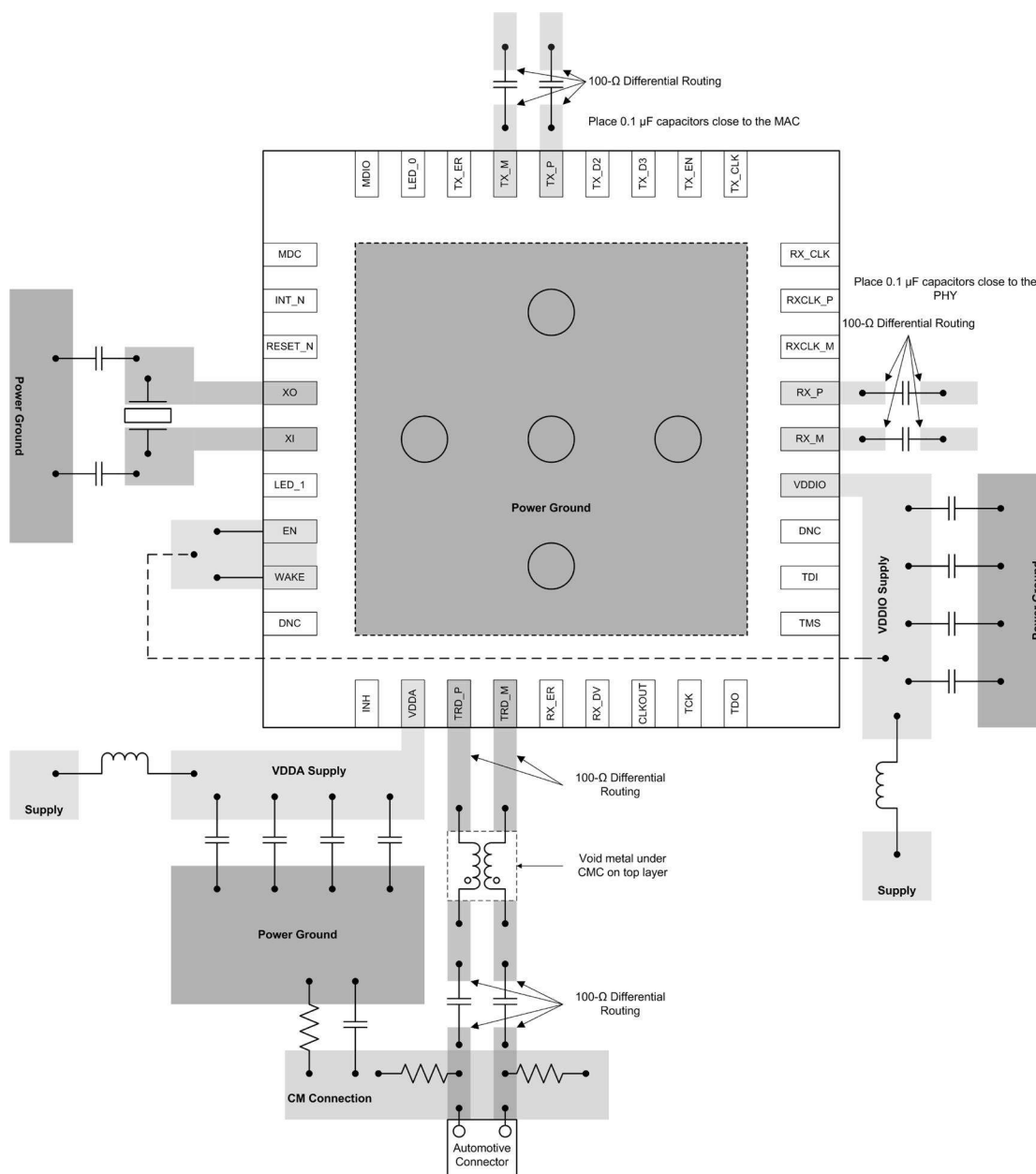
Figure 9-16. DP83TC811SWRHA-Q1 SGMII Layout Recommendation
