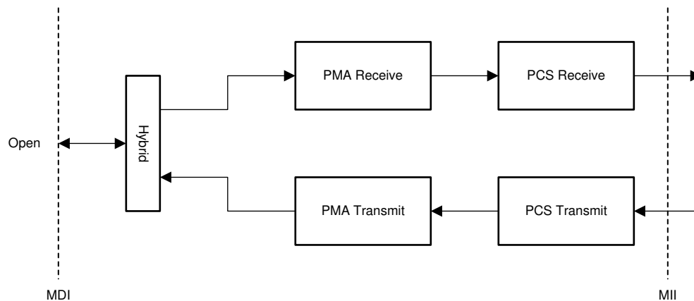
Figure 8-7. Analog Loopback
