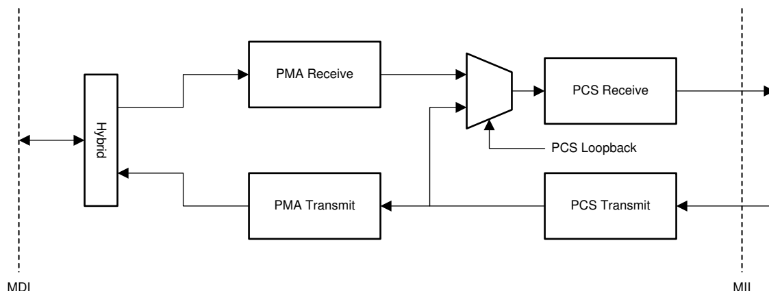
Figure 8-6. PCS Loopback
