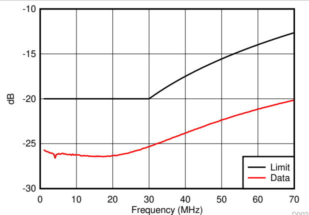
Figure 9-10. MDI Return Loss
