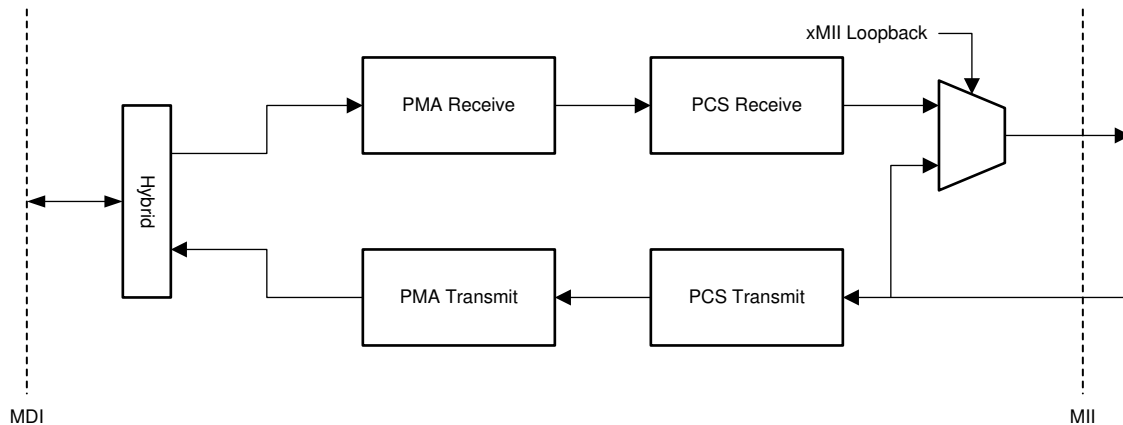
Figure 8-5. xMII Loopback
