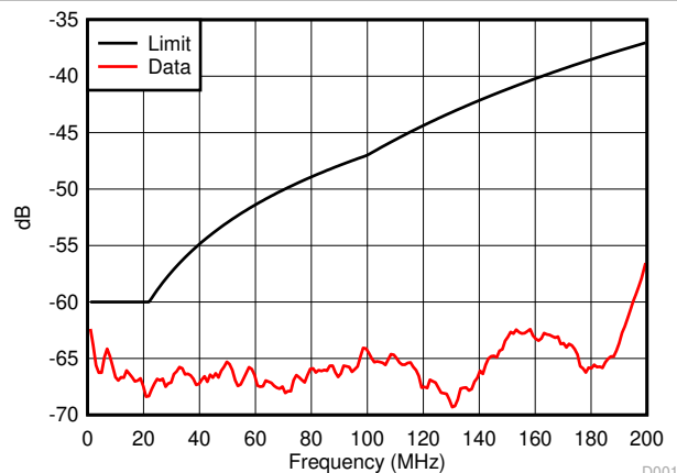
Figure 9-9. MDI Mode Conversion
