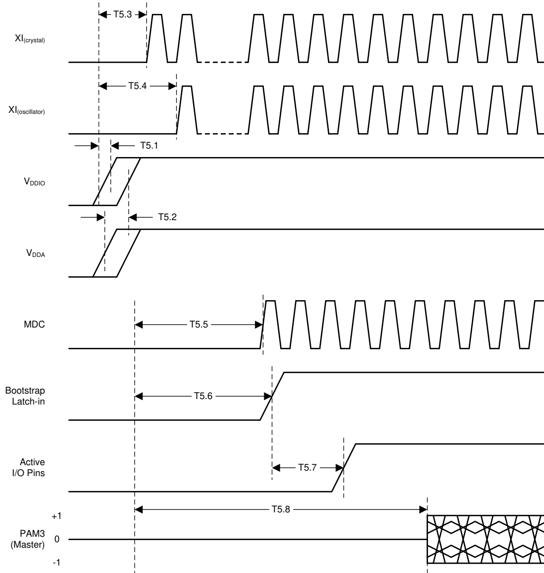
Figure 7-9. Power-Up Timing
