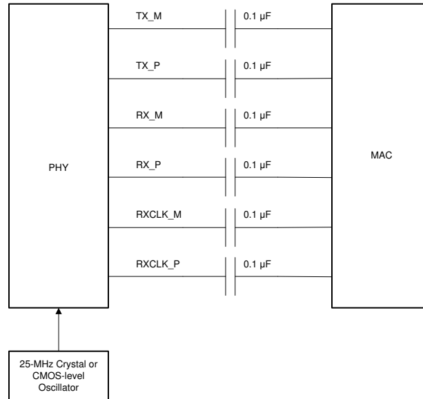
Figure 8-13. SGMII Connections
