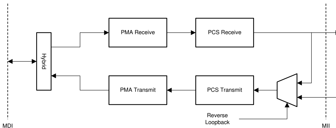
Figure 8-8. Reverse Loopback
