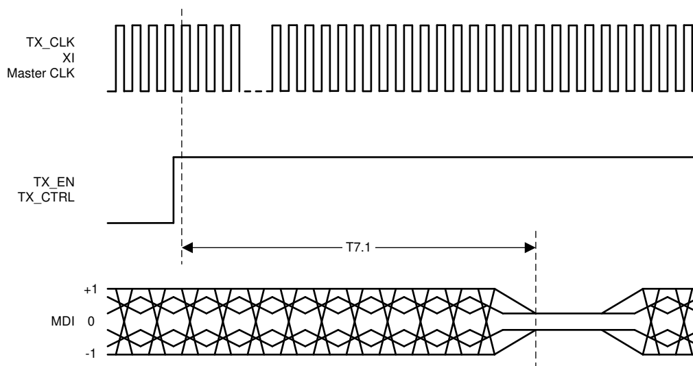
Figure 8-3. Transmit Latency
