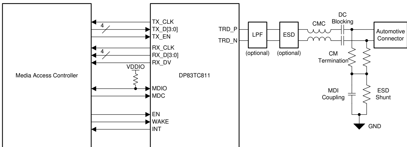
Figure 9-1. Typical Application (MII)
