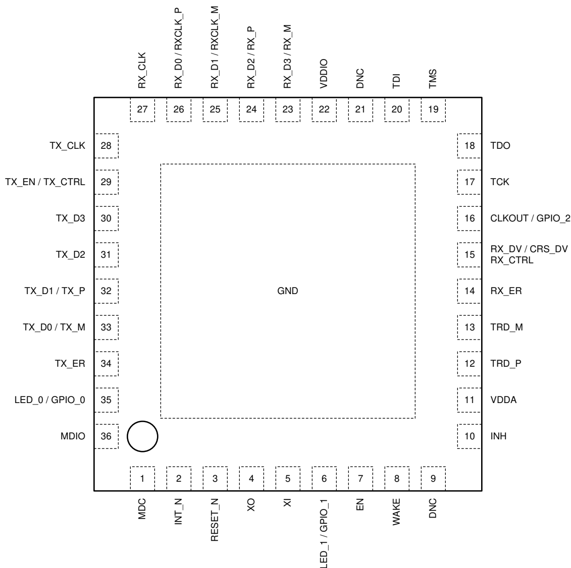
Figure 6-1. RND Package 36-Pin VQFN Top View
