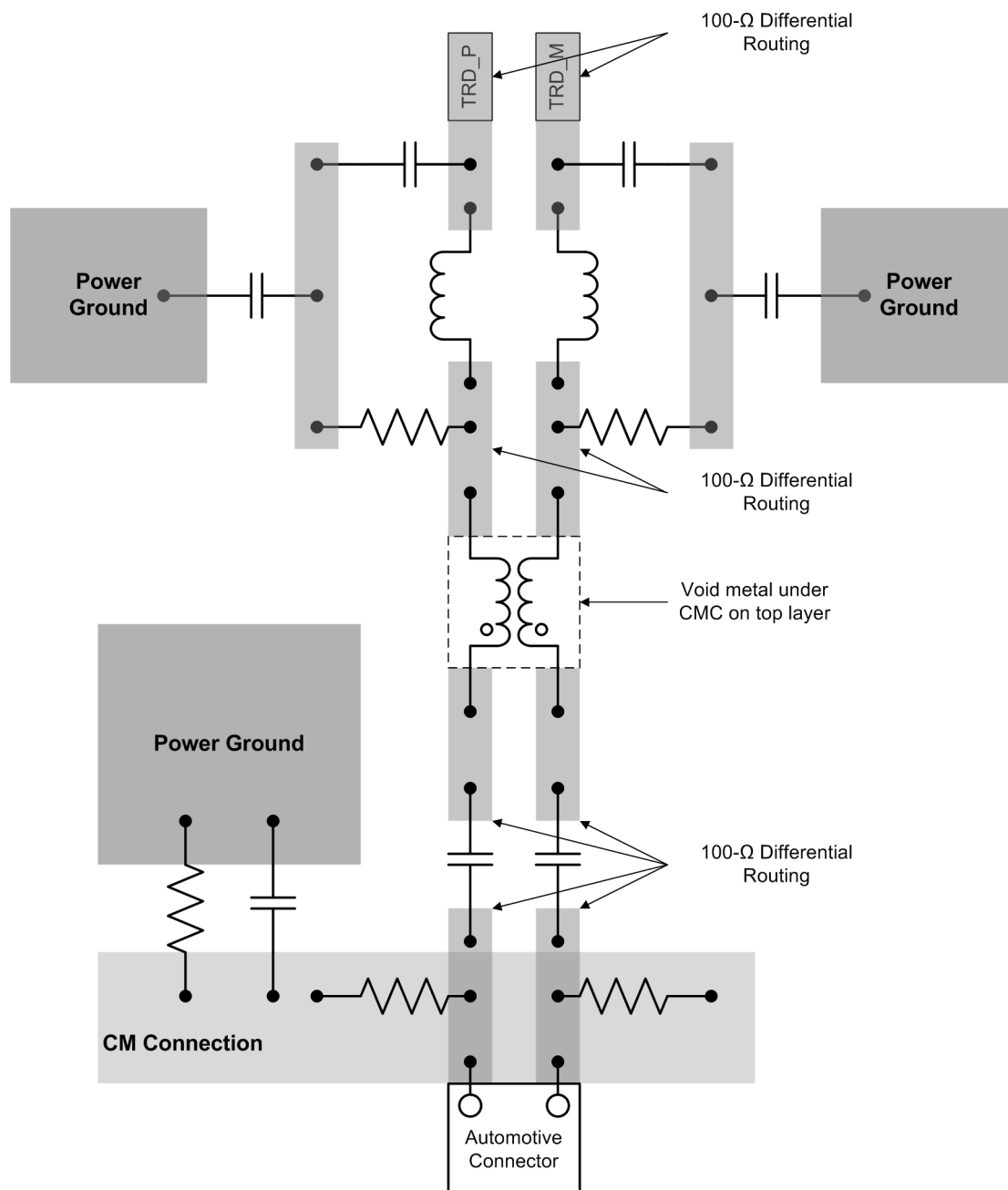
Figure 9-17. MDI Low-Pass Filter Layout Recommendation
