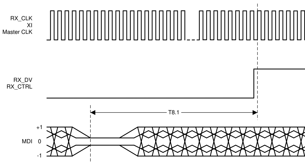
Figure 8-4. Receive Latency
