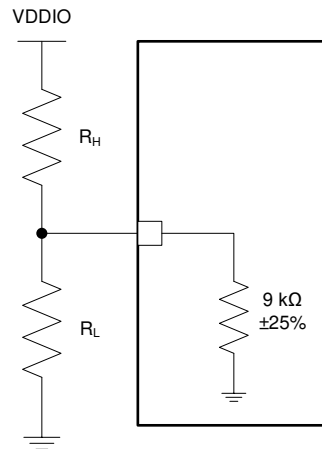
Figure 8-14. Strap Circuit
