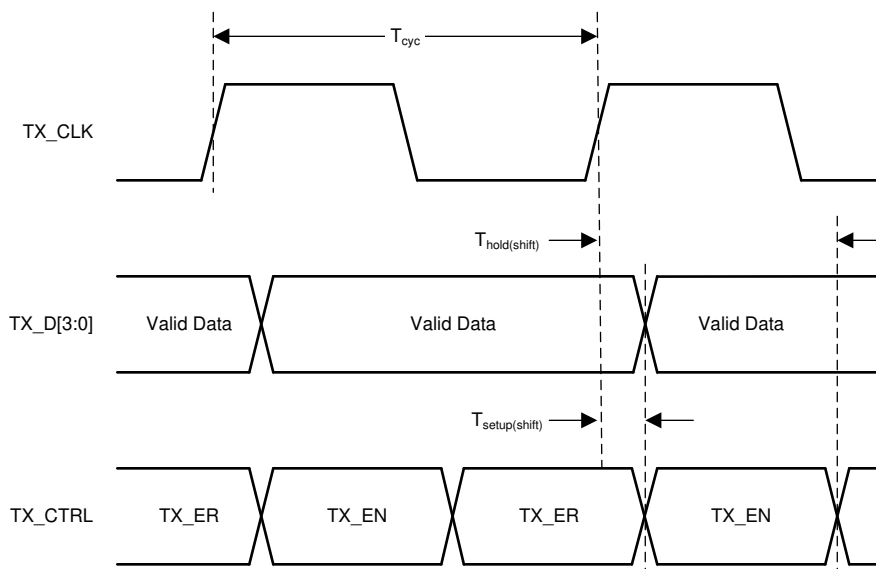
Figure 7-4. RGMII Transmit Timing (Internal Delay Enabled)
