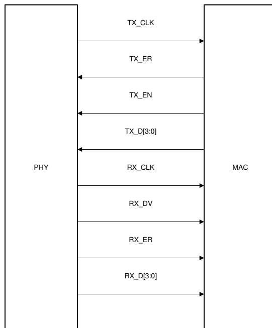
Figure 8-10. MII Signaling
