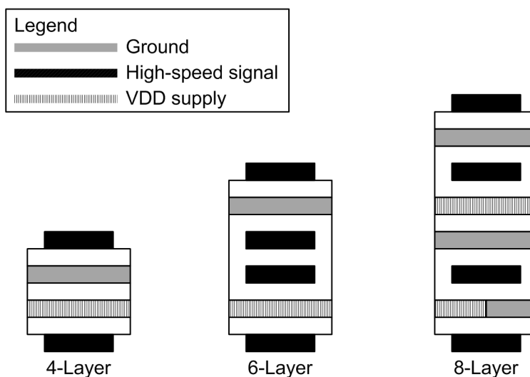
Figure 9-14. Recommended PCB Layer Stack-Up
