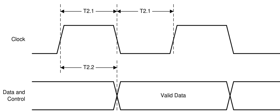
Figure 7-2. MII Receive Timing
