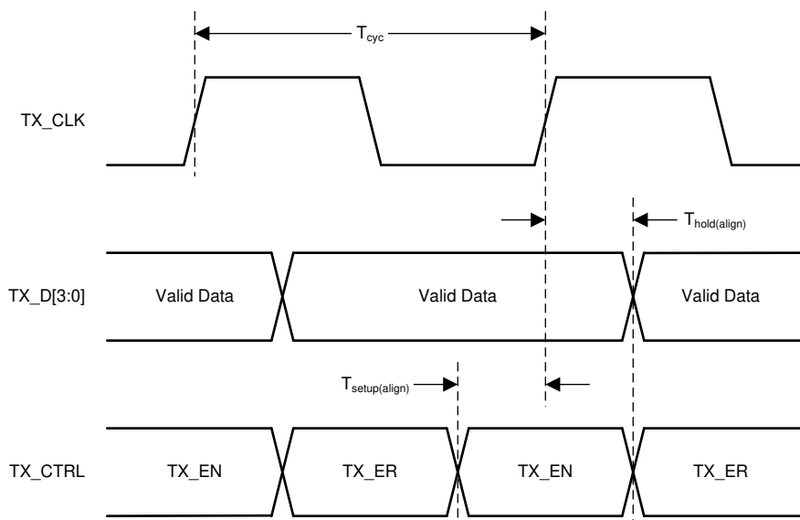
Figure 7-5. RGMII Transmit Timing (Internal Delay Disabled)
