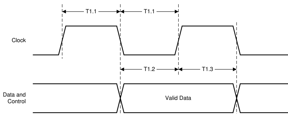
Figure 7-1. MII Transmit Timing
