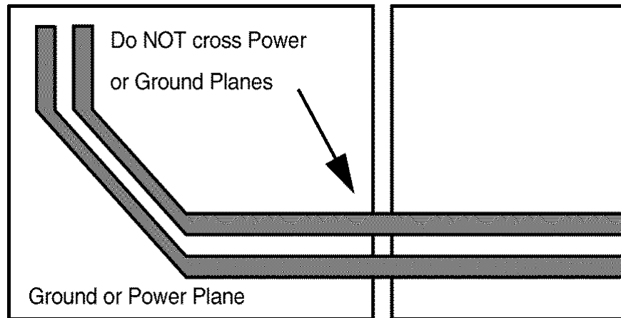
Figure 9-13. Power and Ground Plane Breaks
