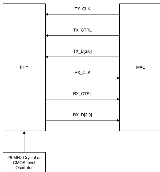
Figure 8-12. RGMII Connections
