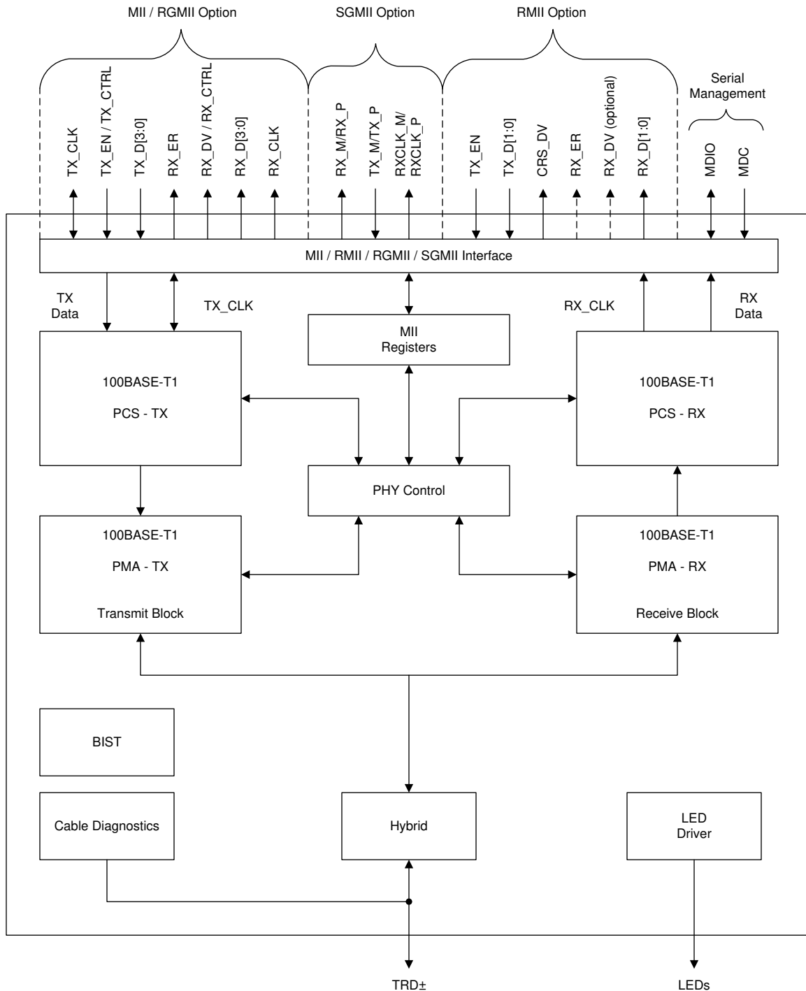
Figure 8-1. DP83TC811-Q1 Functional Block Diagram
