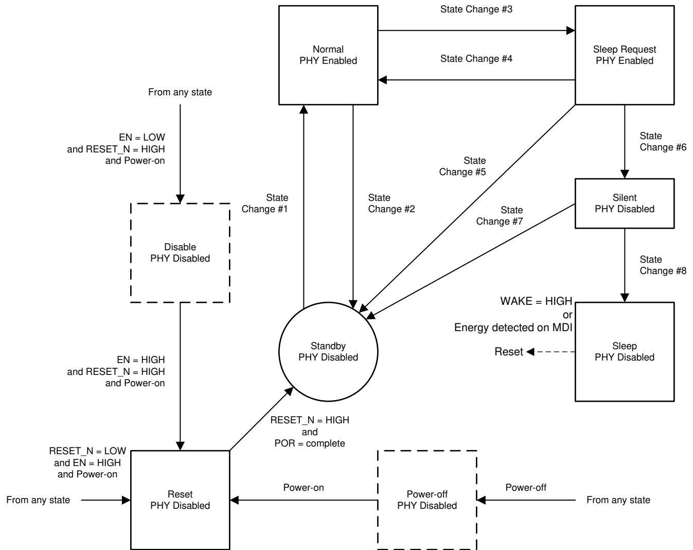
Figure 8-9. PHY Operation State Diagram
