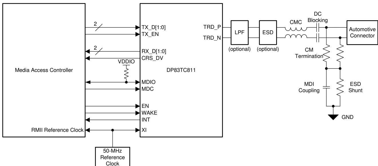
Figure 9-2. Typical Application (RMII Slave)
