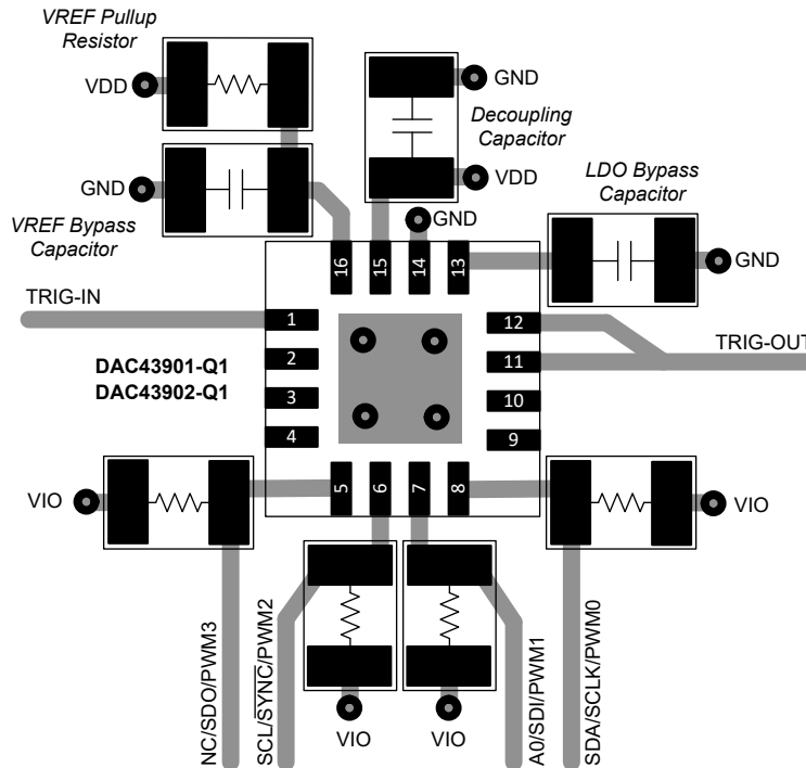
Figure 8-4. Layout Example
