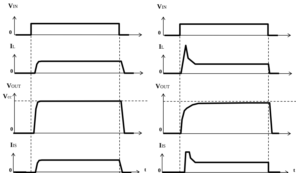
Switching a resistive load
