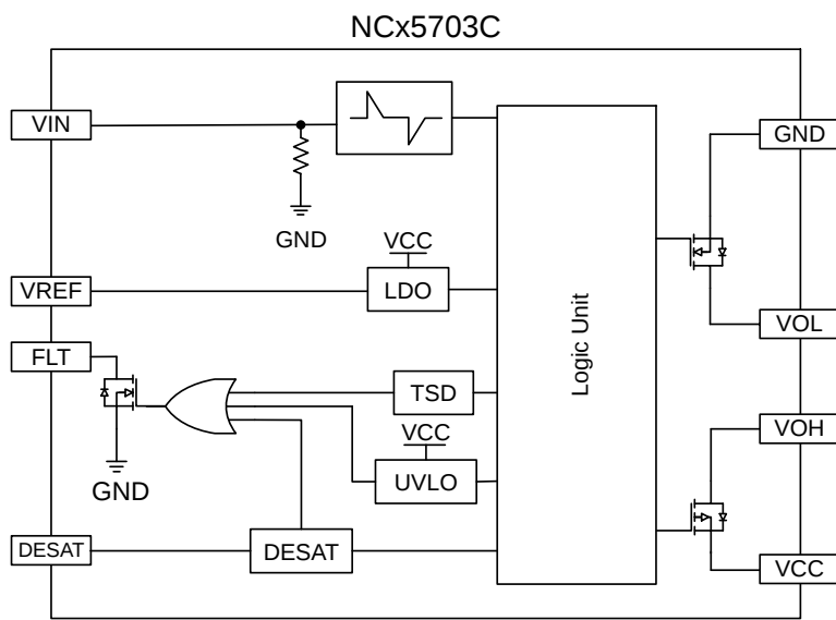
Figure 4(b). Simplified Block Diagram NCx5703C
