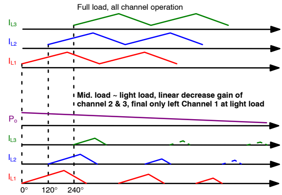
Figure 13. Phase and Gain Change of CM Control
