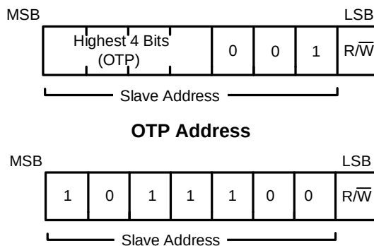
Figure 14: 7-Bit Address
