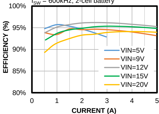
Efficiency vs. Charge Current in Charge Mode
