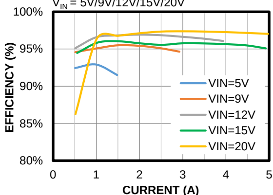
Efficiency vs. Source Current in Source Mode
