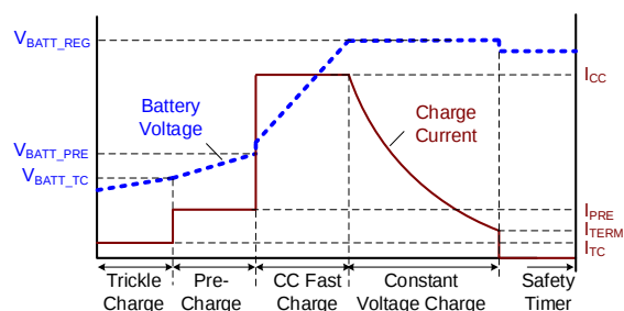
Figure 2: Typical Charge Profile
