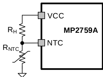
Figure 6: Thermistor Connection
