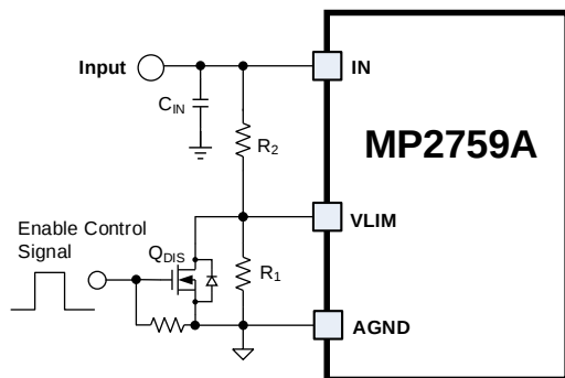
Figure 4: Enable Control
