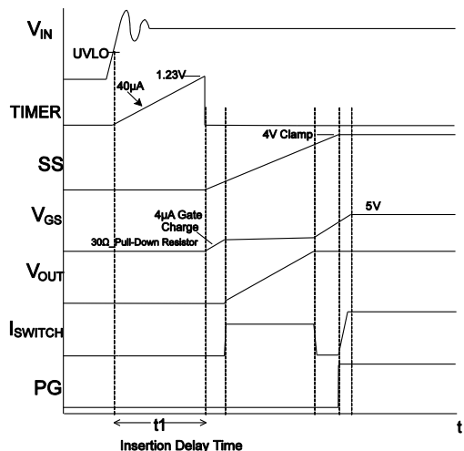
Figure 4: Start-Up Sequence
