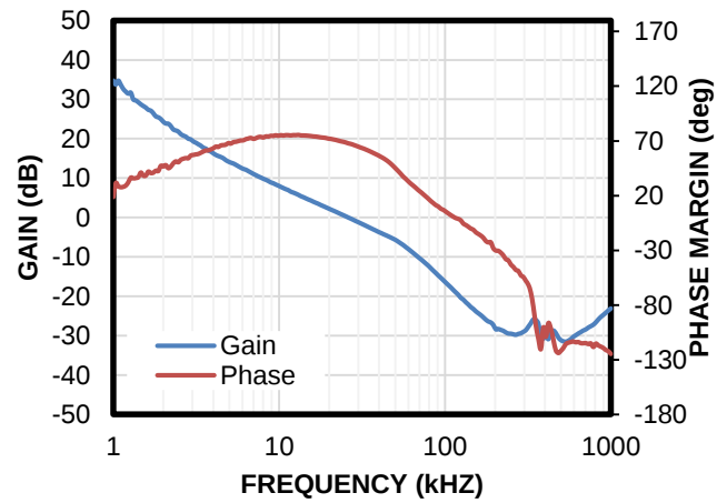
Bode Plot
