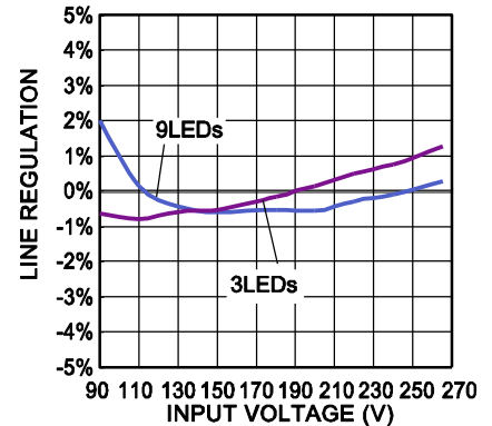
Line Regulation
