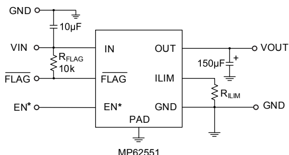
Figure 4: Application Circuit
