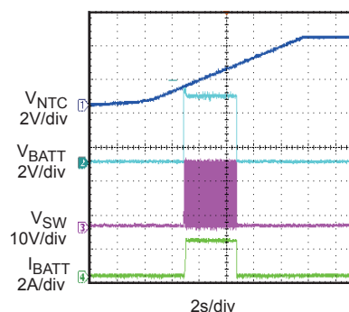
NTC Control
