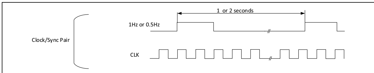
FIGURE 5-5: Reference-Sync Pair.
