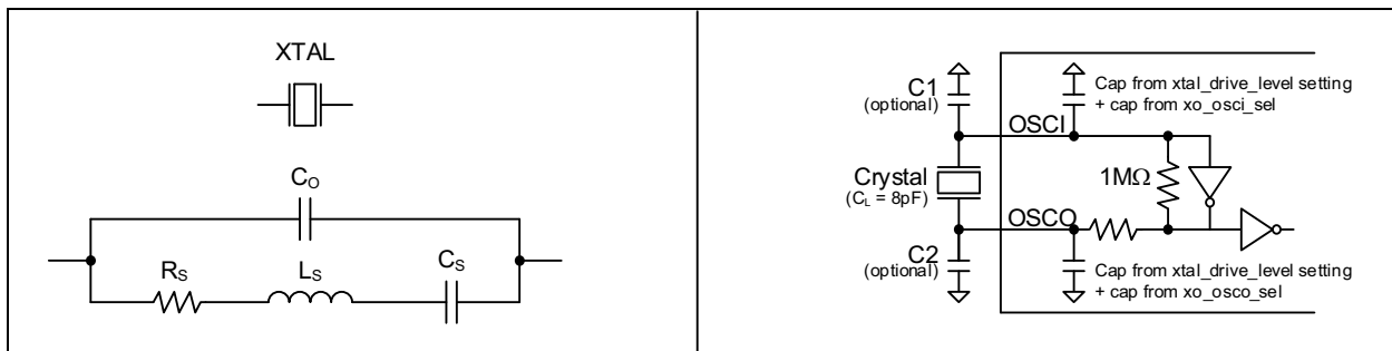
FIGURE 5-8: Crystal Equivalent Circuit/Recommended Crystal Circuit.
