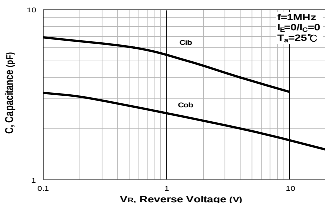
FIG.6 - C_{ob}/C_{ib} - V_{CB}/V_{EB}
