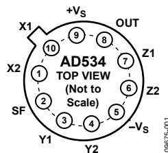
Figure 4. TO-100 (H-10) Pin Configuration
