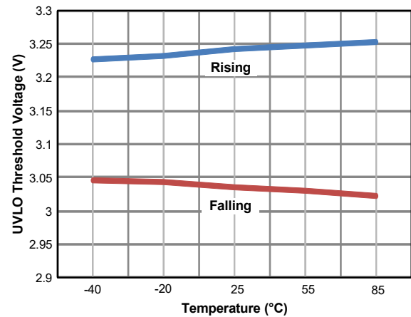
Figure 25. UVLO Threshold vs. Temperature (AOZ1356DI-01, -02)
