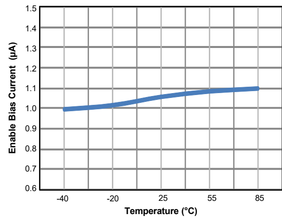
Figure 23. EN Bias Current vs. Temperature
